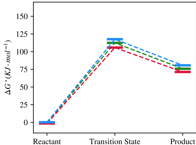
Unperturbed + R/S - water ( \epsilon = 78.4 )
