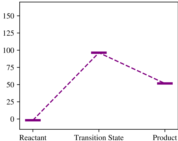
Catalytic - water ( \epsilon_r = 78.4 )
