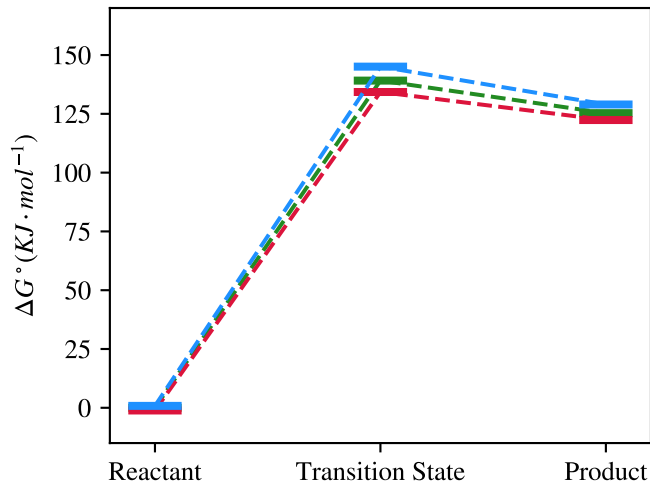
Unperturbed + R/S - hexane ( \epsilon = 2.0 )
