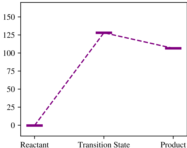
Catalytic - hexane ( \epsilon_r = 2.0 )
