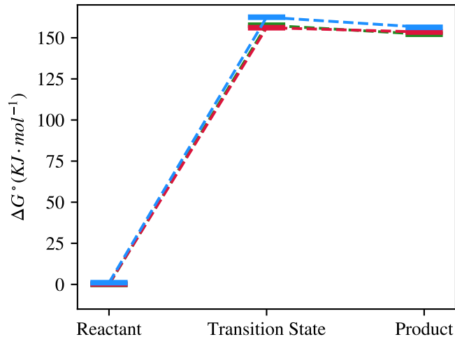
Unperturbed + R/S - gas ( \epsilon = 0.0 )
