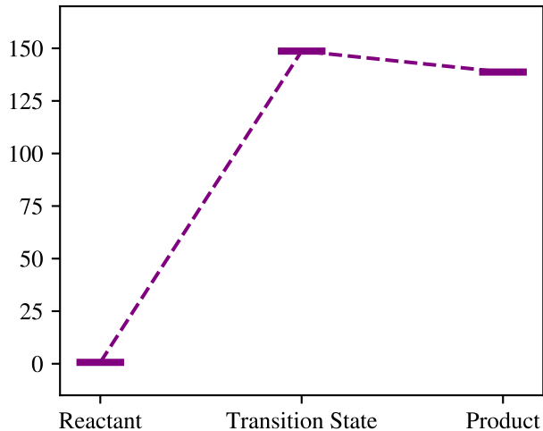
Catalytic - gas ( \epsilon_r = 0.0 )
