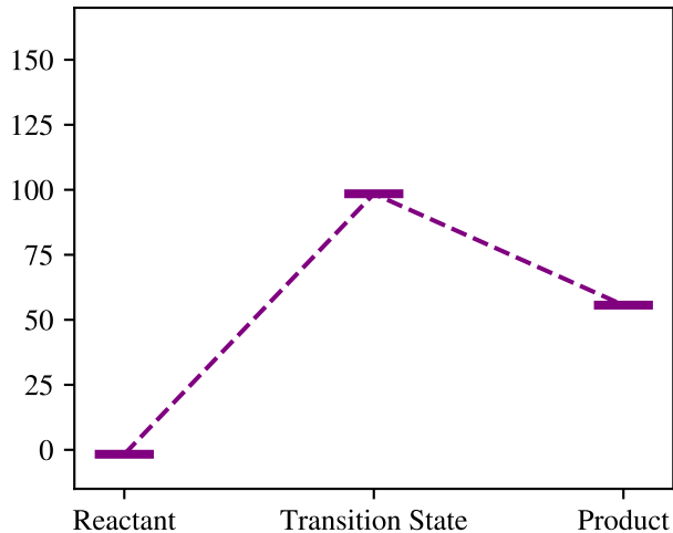
Catalytic - ethanol ( \epsilon_r = 24.9 )
