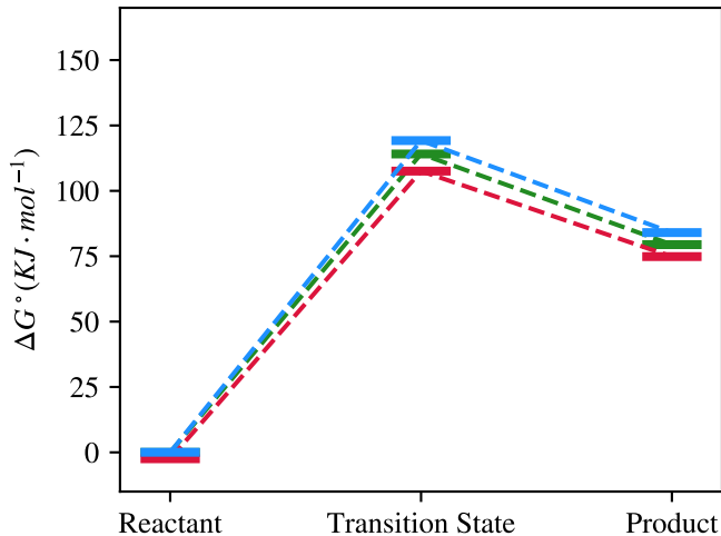
Unperturbed + R/S - ethanol ( \epsilon = 24.9 )
