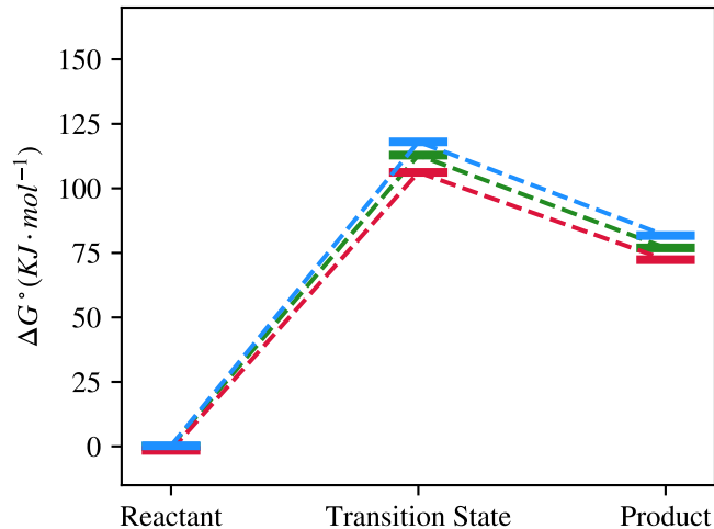
Unperturbed + R/S - dmsO ( \epsilon = 46.8 )
