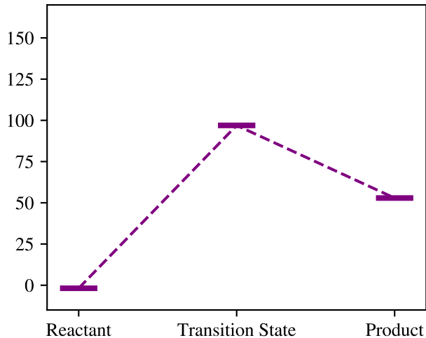
Catalytic - dmsO ( \epsilon_r = 46.8 )
