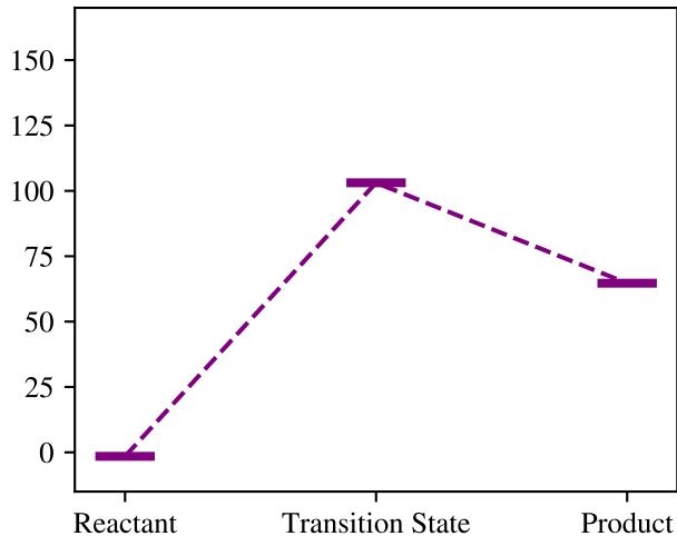
Catalytic - dcm ( \epsilon_r = 8.9 )
