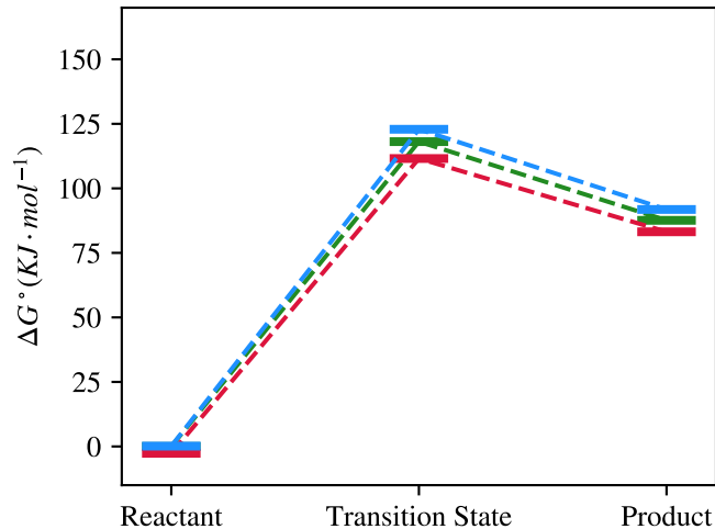
Unperturbed + R/S - dcm ( \epsilon = 8.9 )
